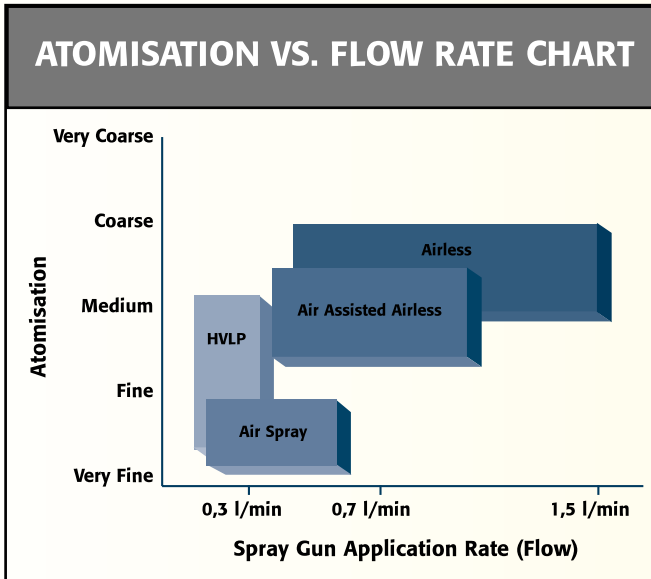
Relative atomisation and typical flow rate comparison of atomisation methods.
